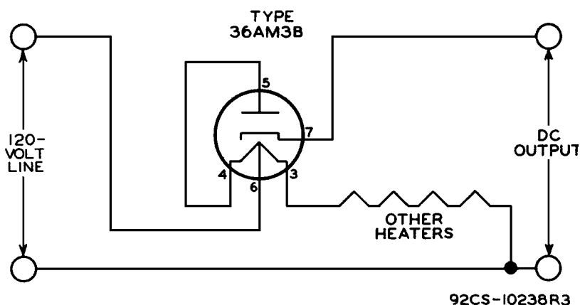
TYPICAL HALF-WAVE CIRCUIT
